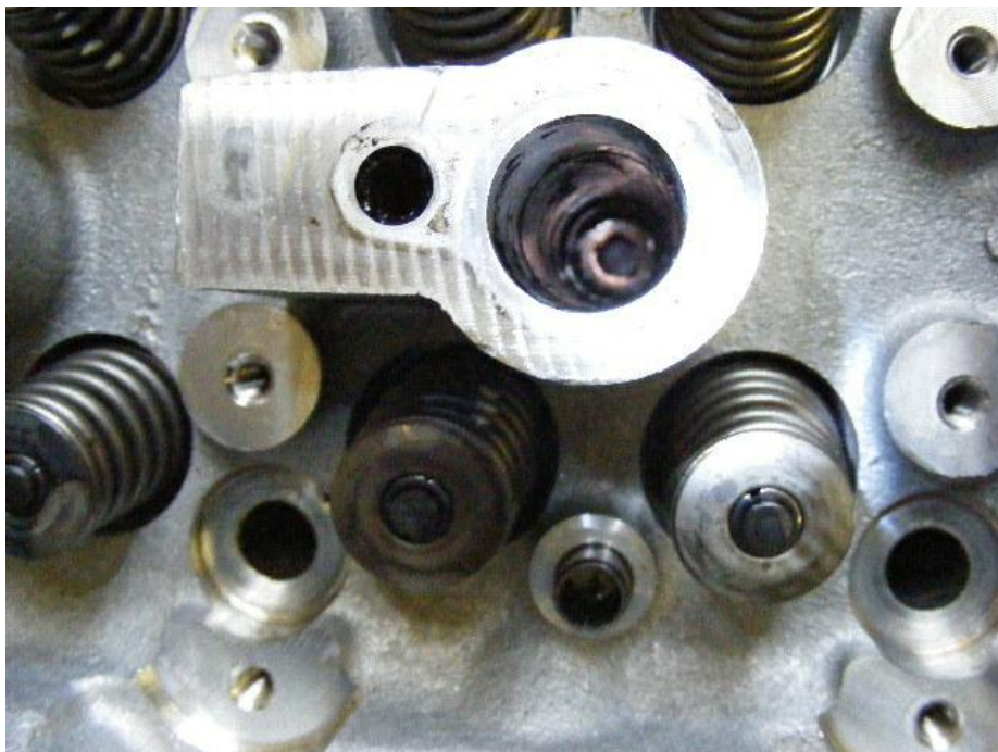
Notice how the copper heat shield washer has been left behind, this will need to be removed so that the cylinder seat can be cleaned.
